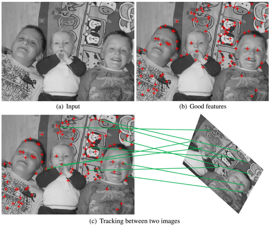
Fig. 9.10 Tracking using SIFT. (a) Input. (b) Each red cross corresponds to the center of a small rectangle containing pixels with high gradient information, i.e., a good region to track. 100 good features are shown. (c) The green lines illustrate where the features have been refound in the new image. Note that only ten features are shown to increase visibility
