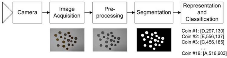
Fig. 13.3 The block diagram of the image processing part of the system. The output for each coin is its type and center
