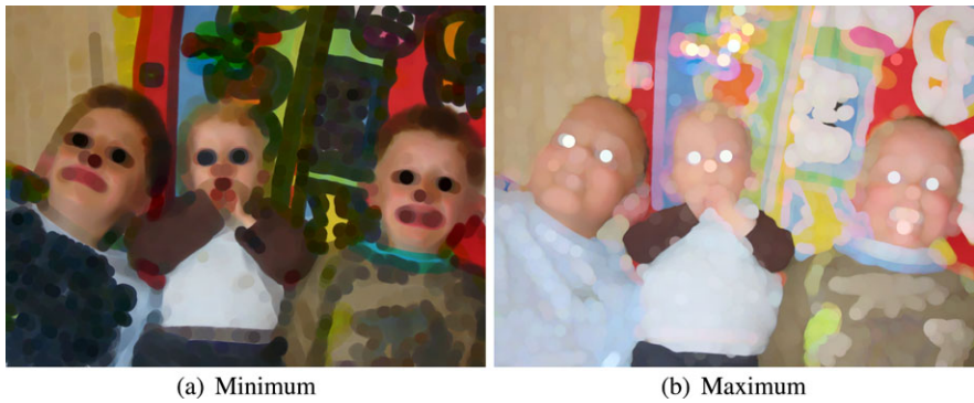
Fig. 11.5 Rank filters
