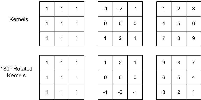
Fig. 5.19 Three kernels and their rotated counterparts
