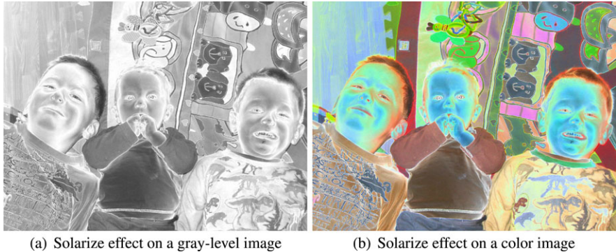
Fig. 11.4 Solarize filter
